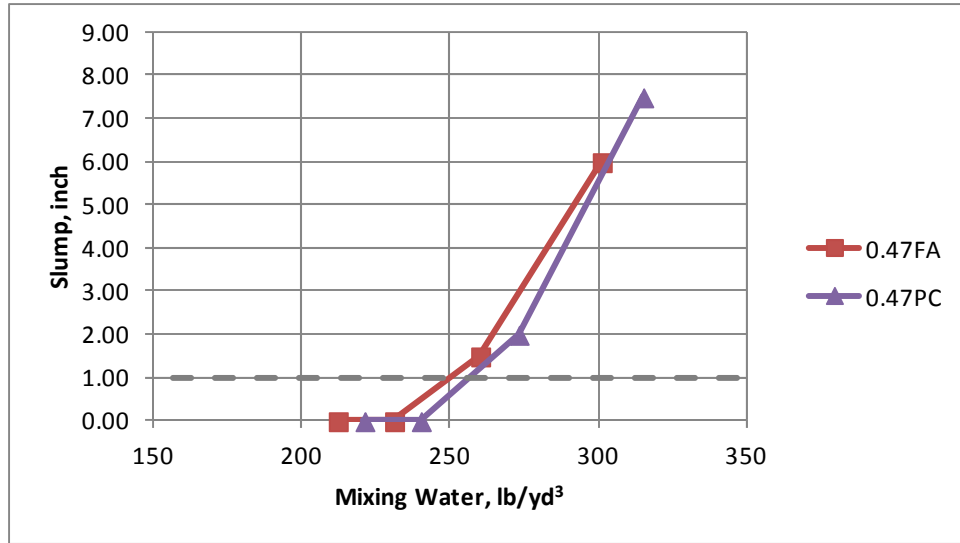
Figure 2: Phase I: Measured Slump for the Portland Cement and Fly Ash Mixtures prior to adding any HRWRA Vs Mixing Water Content
