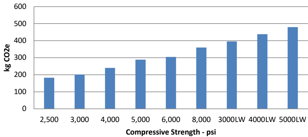
Figure B2-Climate Change-GWP
