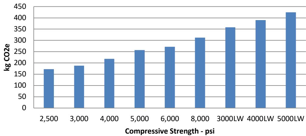
Figure B8-Climate Change-GWP
