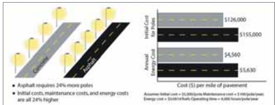
Figure 2. Cost and light pole differential between concrete and asphalt roadways. Reprinted from “Enlightened” (QD-010P), a publication of the American Concrete Pavement Association. ©2007, American Concrete Pavement Association. All rights reserved.
